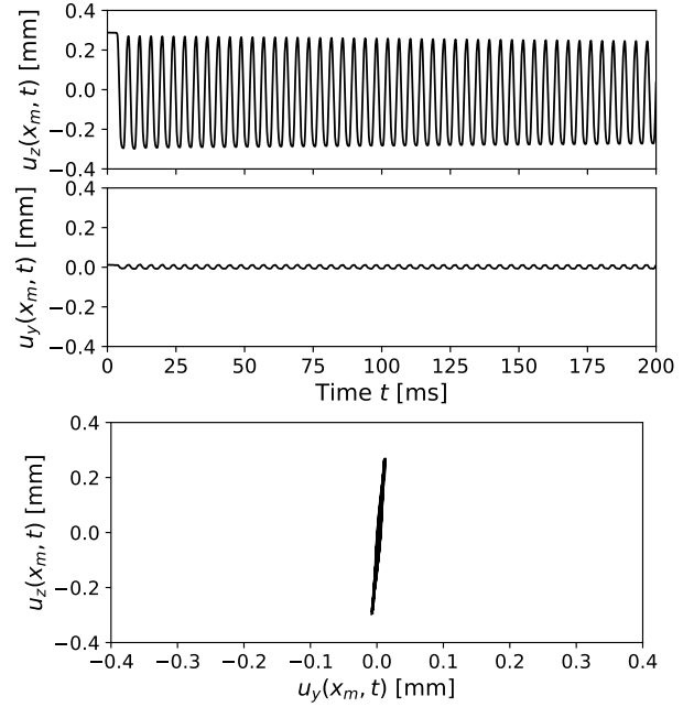
Figure 6. Persistent planar vibration. String displacement u is recorded at x = x_m using the measurement set-up shown in Fig. 4. Subscripts y and z indicate the direction of vibration as shown in Figs. 1 and 4.
