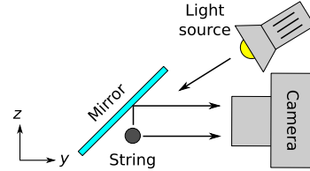
Figure 4. Dual polarisation measurement set-up [15].
